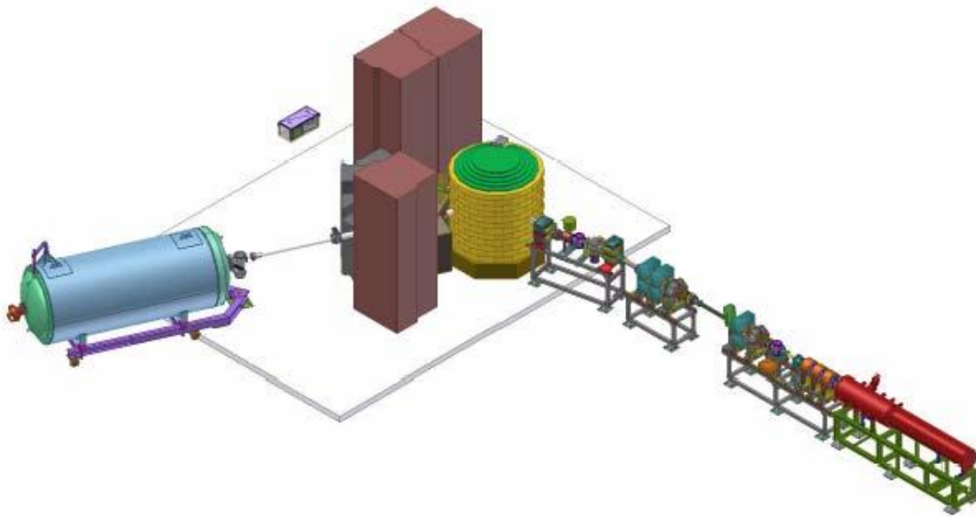
Figure 1: Overall schematic layout for LENS Phase I. Shown are the accelerator (right-hand of the picture), the TMR (vertical cylinder at the center of the picture), the SANS instrument, and the camera on the radiography station.
