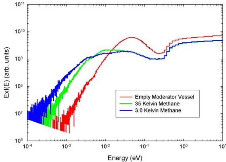
Figure 5: Neutron spectra collected after the installation of the cryogenic methane moderator. These spectra were taken with a high-efficiency ^3\text{He} detector that viewed the source through a 5x20mm hole in a Cd mask in order to avoid saturation effects. The empty moderator spectrum was collected with the moderator vessel at a temperature of 130K after all methane had been removed. The 3.6K spectrum was collected with the moderator filled with methane and a small amount of liquid helium (the latter used to enhance thermal contact to the vessel). The intermediate curve was collected at a time when the moderator vessel temperature had risen to 35K. In this case, the actual temperature of the methane may be somewhat lower, as the methane was probably decoupled thermally from the vessel after the helium was removed.
