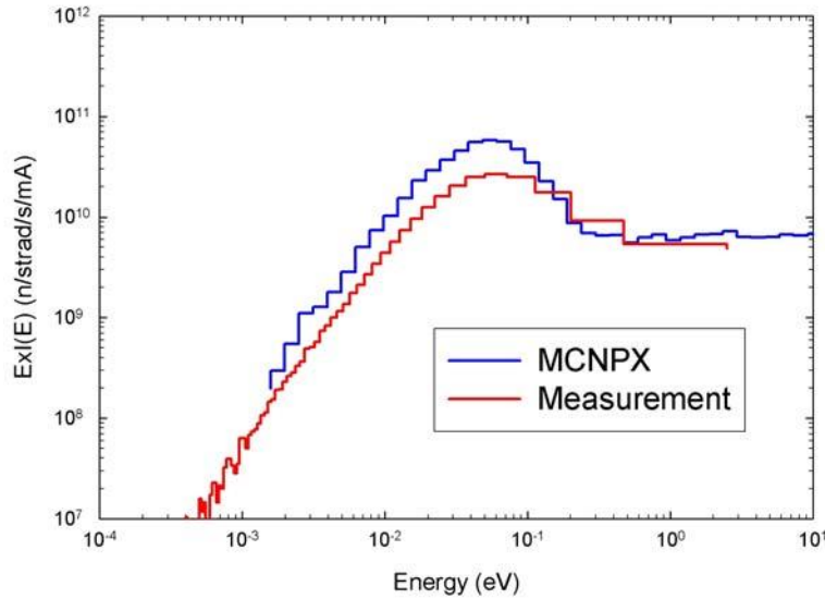
Figure 4: Comparison of a thermal neutron spectrum measured at LENS when operating at 7MeV with that predicted from MCNP calculations. The measurements were taken for a simple room-temperature polyethylene moderator and the measurements made with a flat geometry, low-efficiency ^3\text{He} detector positioned 5.7m from the source and normalized with a set of bare and Cd-covered In activation foils positioned 1.4m from the source.
