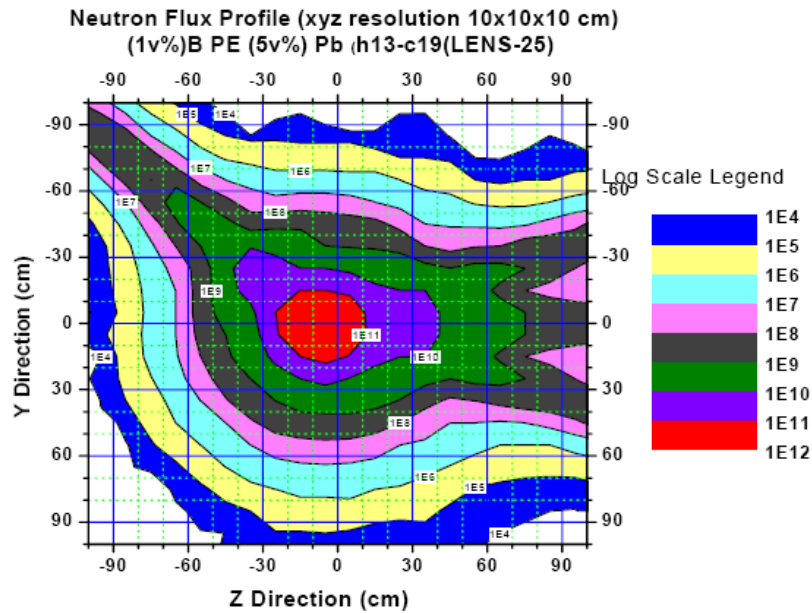
Figure 2: Displayed is the total neutron flux distribution in the equatorial plane of the LENS TMR when the source is operating at 13MeV and 32kW beam power as predicted by MCNP. In this view the proton beam enters in from the upper left corner and three neutron beams are extracted toward the right hand side. The methane moderator is centered at the origin and the Be target is positioned at z = -9\text{cm} , y = 0\text{ cm} .
