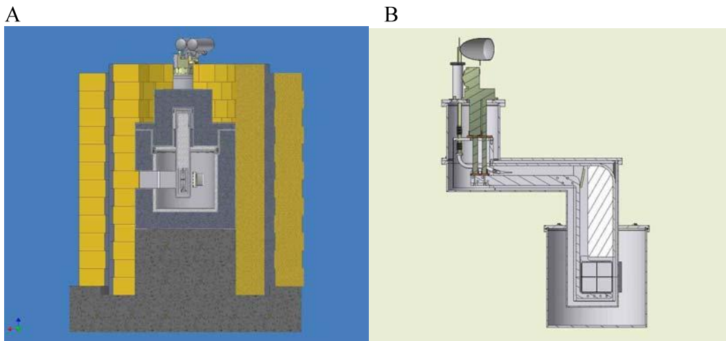
Figure 3: A,B Cross Sectional views of the LENS TMR assembly. The proton beam comes in from the right in figure A, and the neutrons are fed out to instruments on the left. Figure B shows details of the thermal connection between the closed-cycle refrigerator and the methane moderator at the center of the water reflector (which is 50cm in diameter). In B, the white hatched area is a polyethylene plug designed to limit neutron streaming upward and the high-purity Al thermal link is the gray hatched material to its left.
